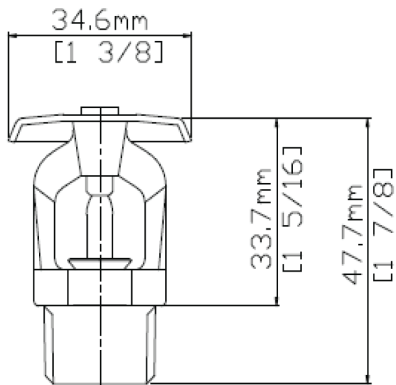
UPRIGHT SPRINKLER
