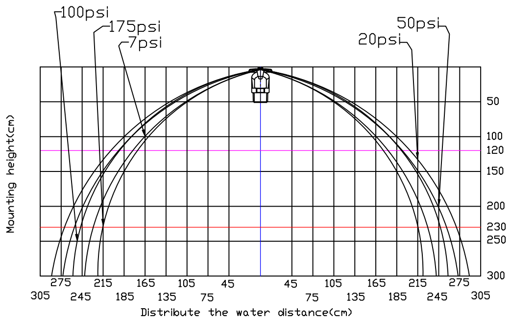
K5.6 UPRIGHT SPRINKLER DISTRIBUTION PATTERNS - TRAJECTORY
