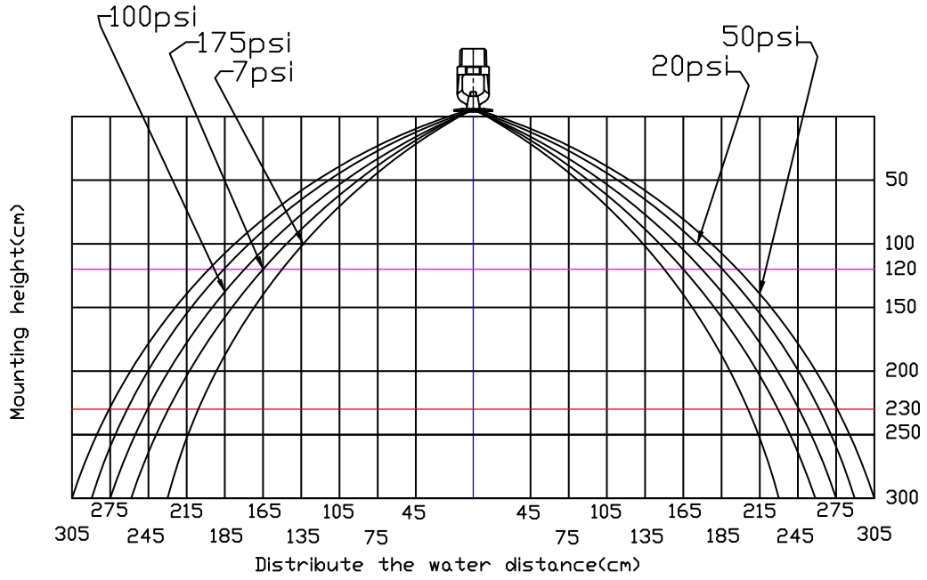
K5.6 PENDENT SPRINKLER DISTRIBUTION PATTERNS - TRAJECTORY
