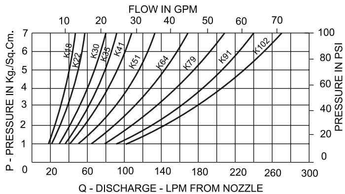
DISCHARGE CHARACTERISTICS
