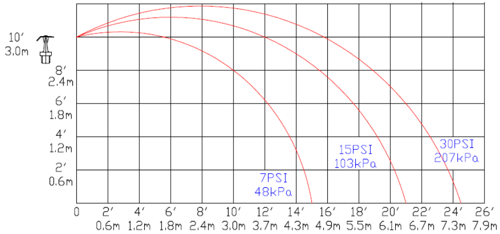
K5.6 STANDARD VERTICAL SIDEWALL DISTRIBUTION PATTERNS - PLAN VIEW
