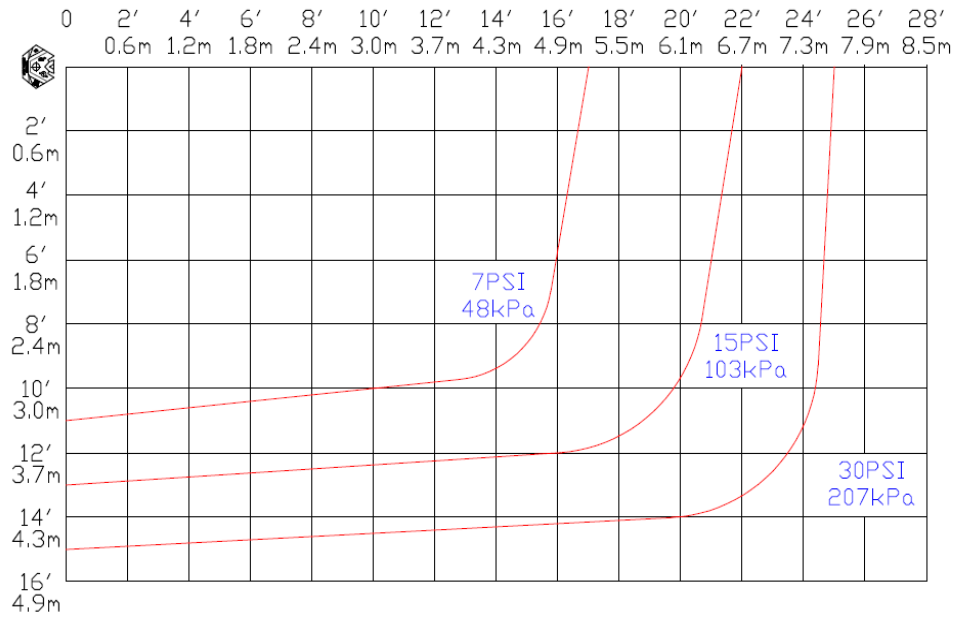
K5.6 STANDARD VERTICAL SIDEWALL DISTRIBUTION PATTERNS - TRAJECTORY
