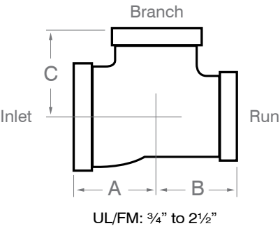
SDT-53 Reducing Tee
